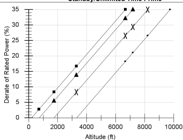
1,800 RPM Power Derate Curves Standby/Unlimited Time Prime
